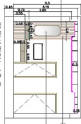
ELEVATION AT B
